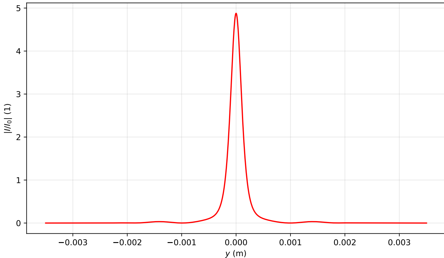
Intensity profile I(x=0, y, z=2.388)/I_0 , P_{in}=2.0P_{cr} , artificial time
